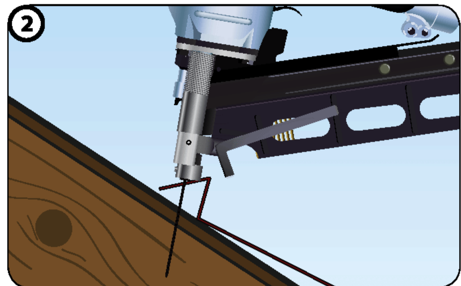
2 Back Flange is seated down onto roof deck.
