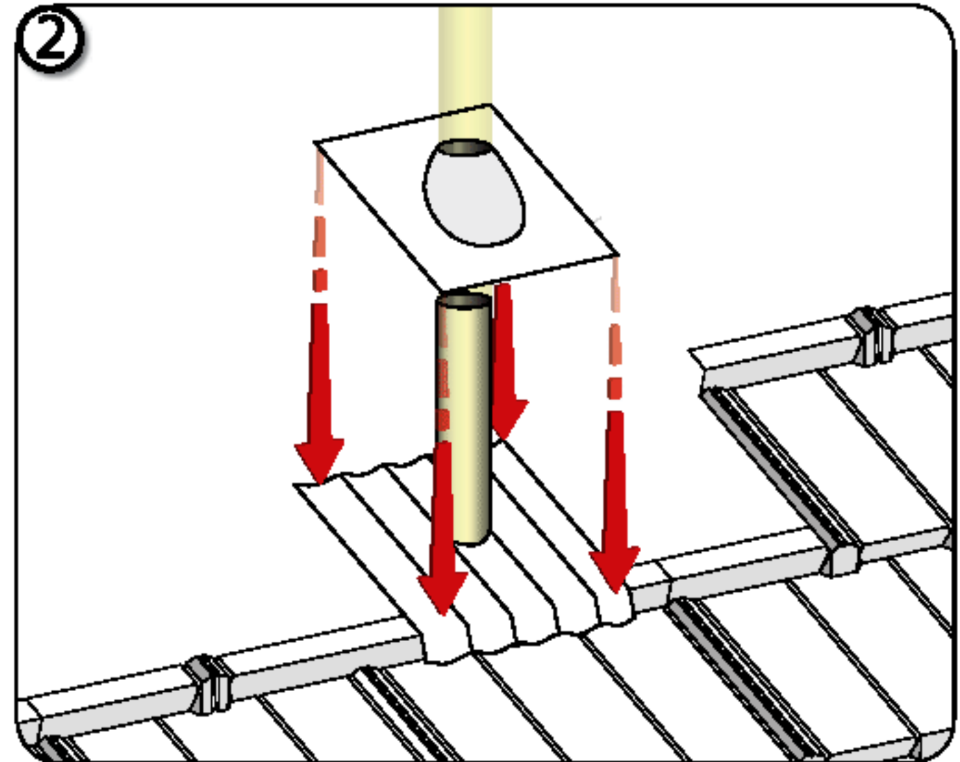
2 Install pipe flashing over 'Under-Pan'.
