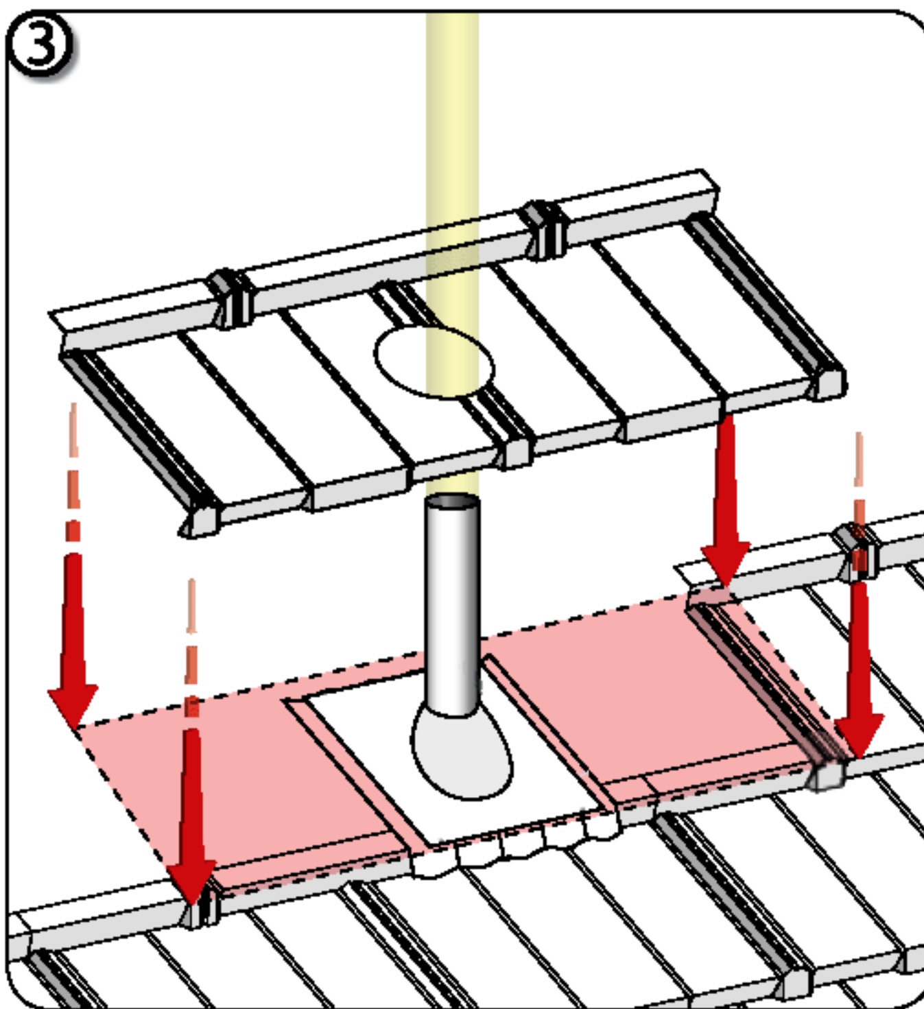
3 Cut a hole in the covering panel to fit the cone of the Pipe Flashing.
