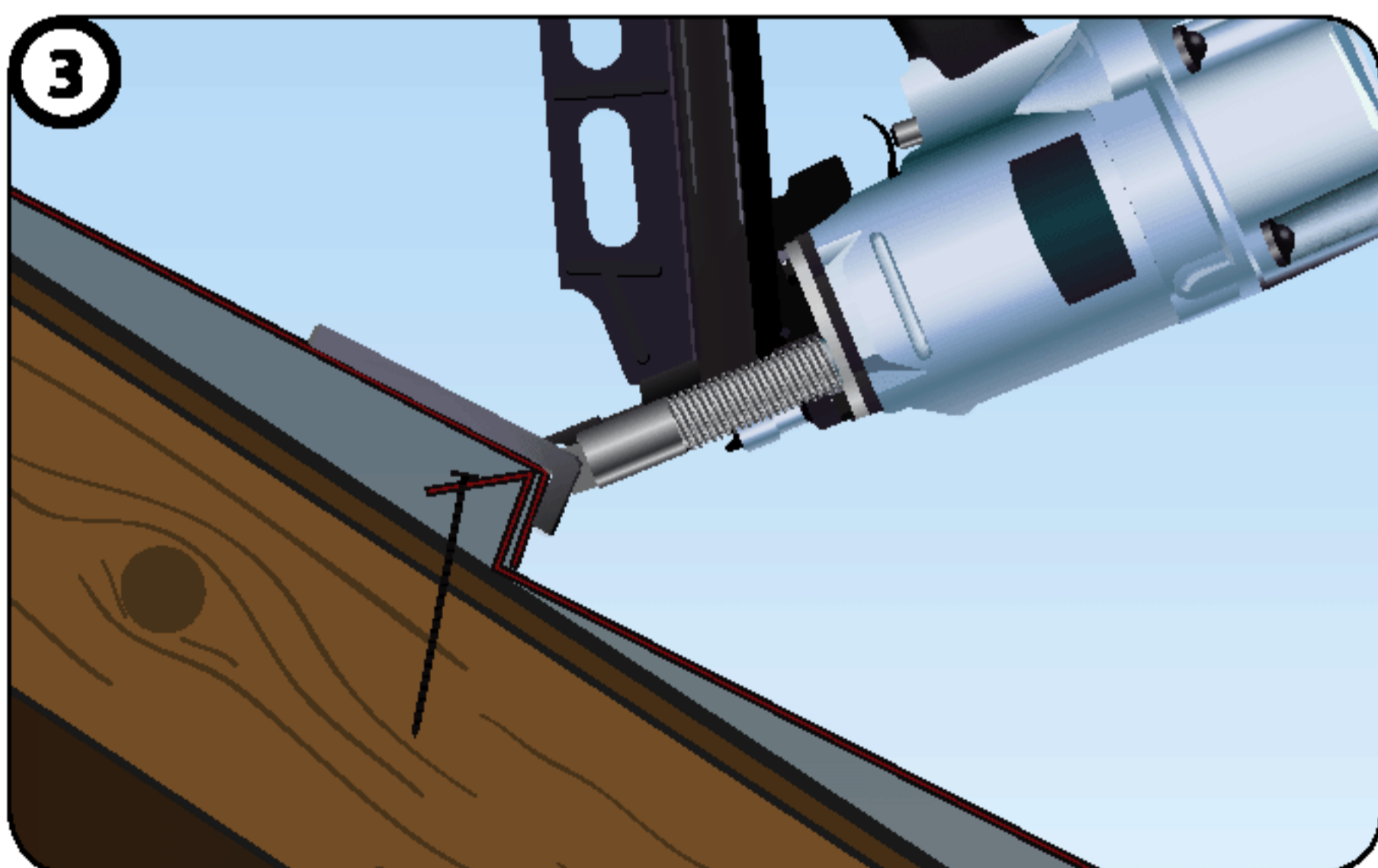
3 Install nose fasteners at an approximate 60-degree angle.
