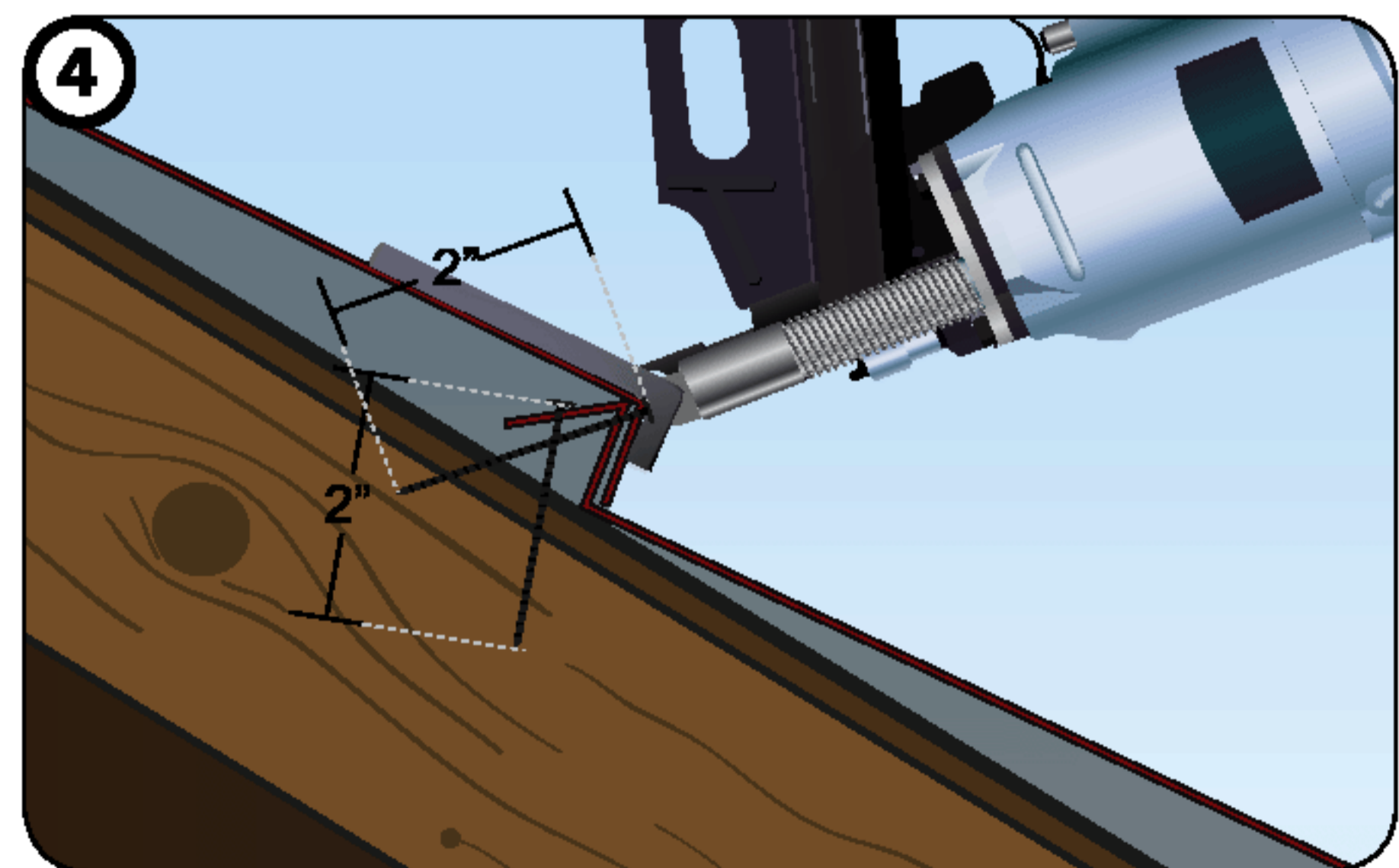
4 Use of the nail-gun attachment ensures correct nose-nail fastener angle.
