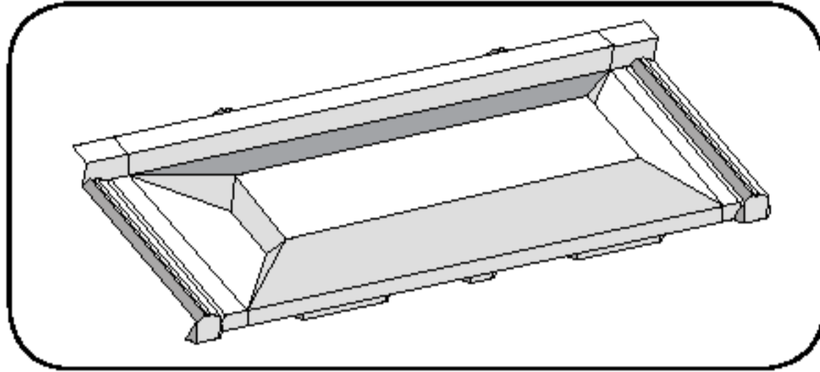
MetroShake SMARTvent 52" x 14.5" x 3.5" - 10.5 lbs. Net Free Vent Area 82.5"
