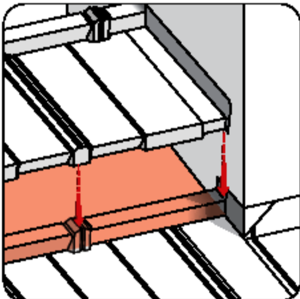
Install subsequent panels with a 2" bend up nested against the protrusion.
