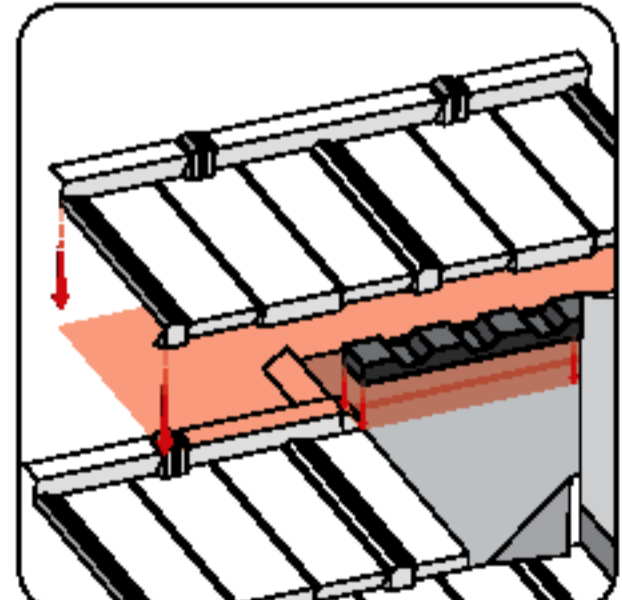
For added protection install a foam weather block as shown to seat the panel onto.
