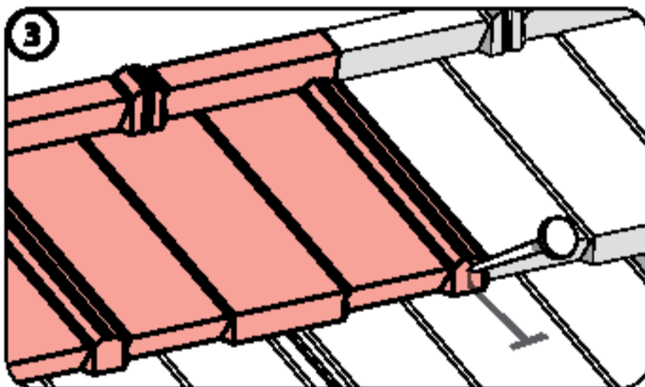
Fasten bottom right corner
