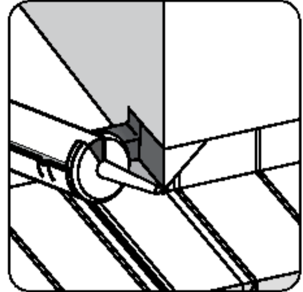
Cut and fold up panels 2" at sides of protrusion as shown.
