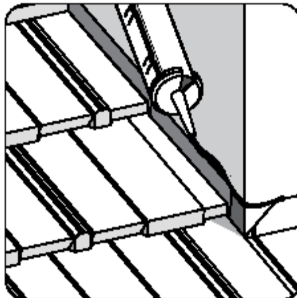
Seal around perimeter of folded panels prior to fastening them to the protrusion.
