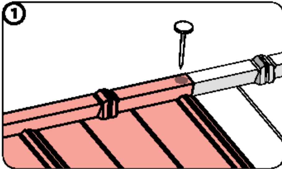
Fasten top right corner
